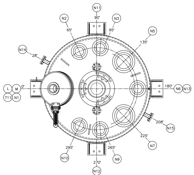
NOZZLE ORIENTATION AE-4000L TO AE-6300L
