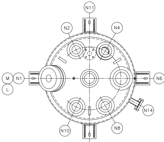
NOZZLE ORIENTATION AE-63L TO AE-630L
