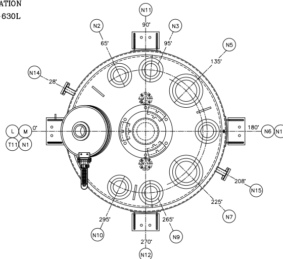
NOZZLE ORIENTATION AE-4000L TO AE-6300L
