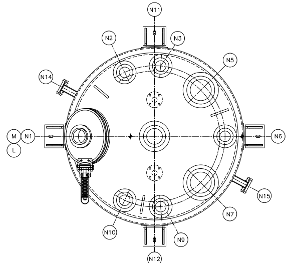
NOZZLE ORIENTATION AE-1000L TO AE-3000L
